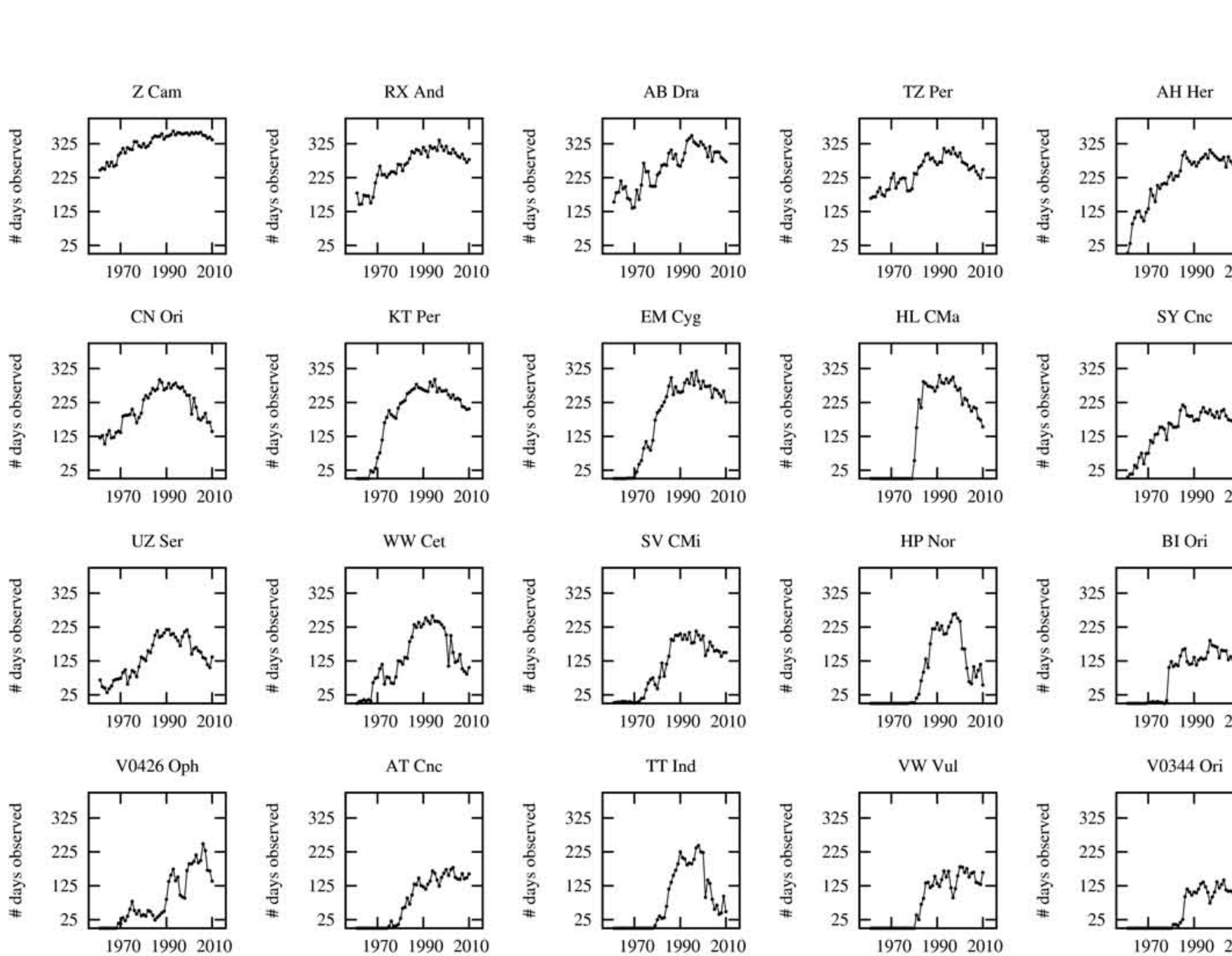
Figure 5: The 20 best-observed dwarf novae of type UGZ (Z Cam-type). Z Cam itself is well observed but as with the UGSS stars, the UGZs show generally declining coverage in the past 5-10 years.
