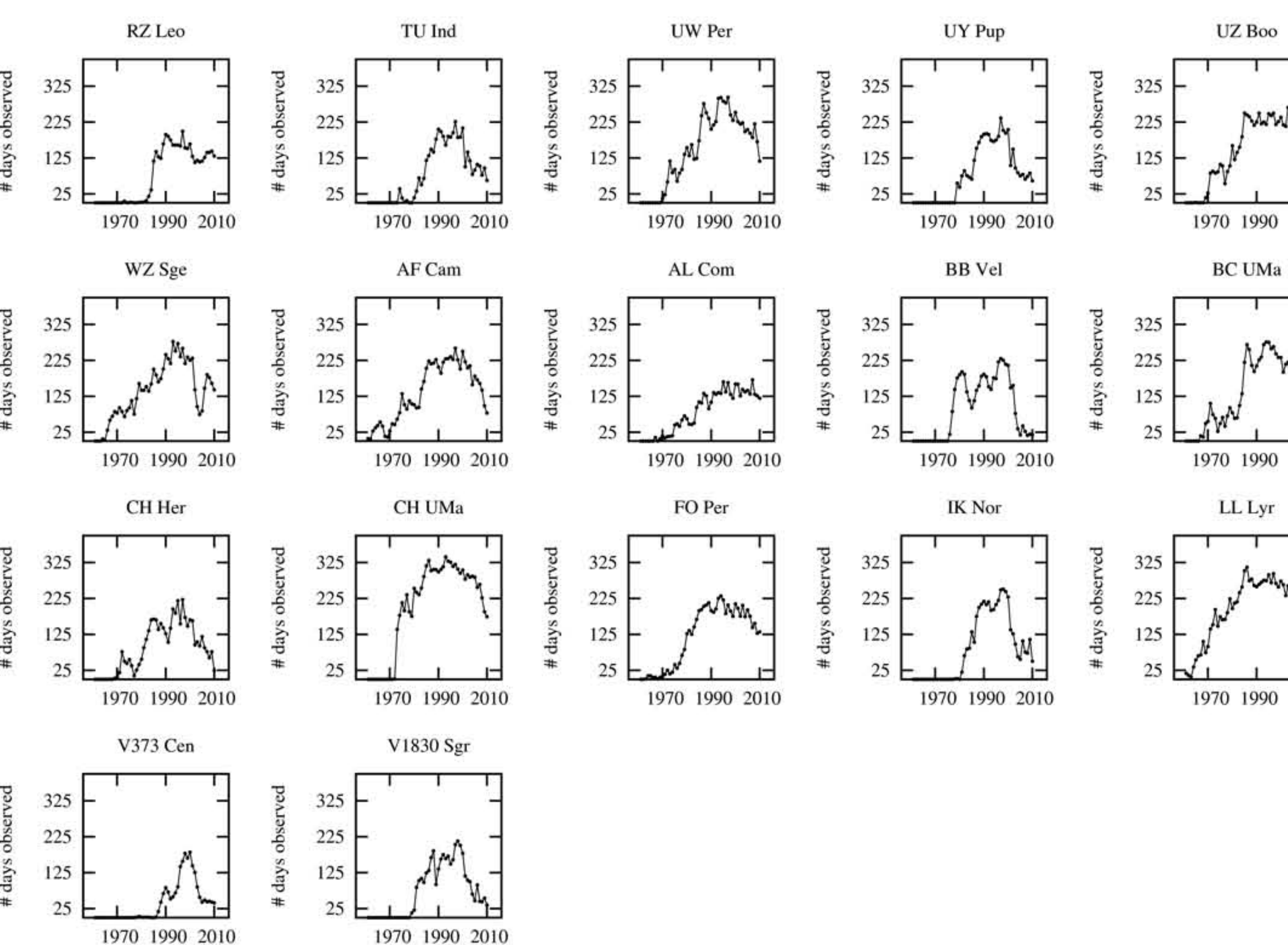
Figure 6: Seventeen well-observed dwarf novae of miscellaneous types, primarily UGWZ (WZ Sge-type). Few of these stars have been extensively observed for many decades, although UZ Boo appears to receive consistent coverage for about 75% of the year. Coverage of UGWZ stars with marginally predictable recurrence times may decline outside of expected outburst windows.
