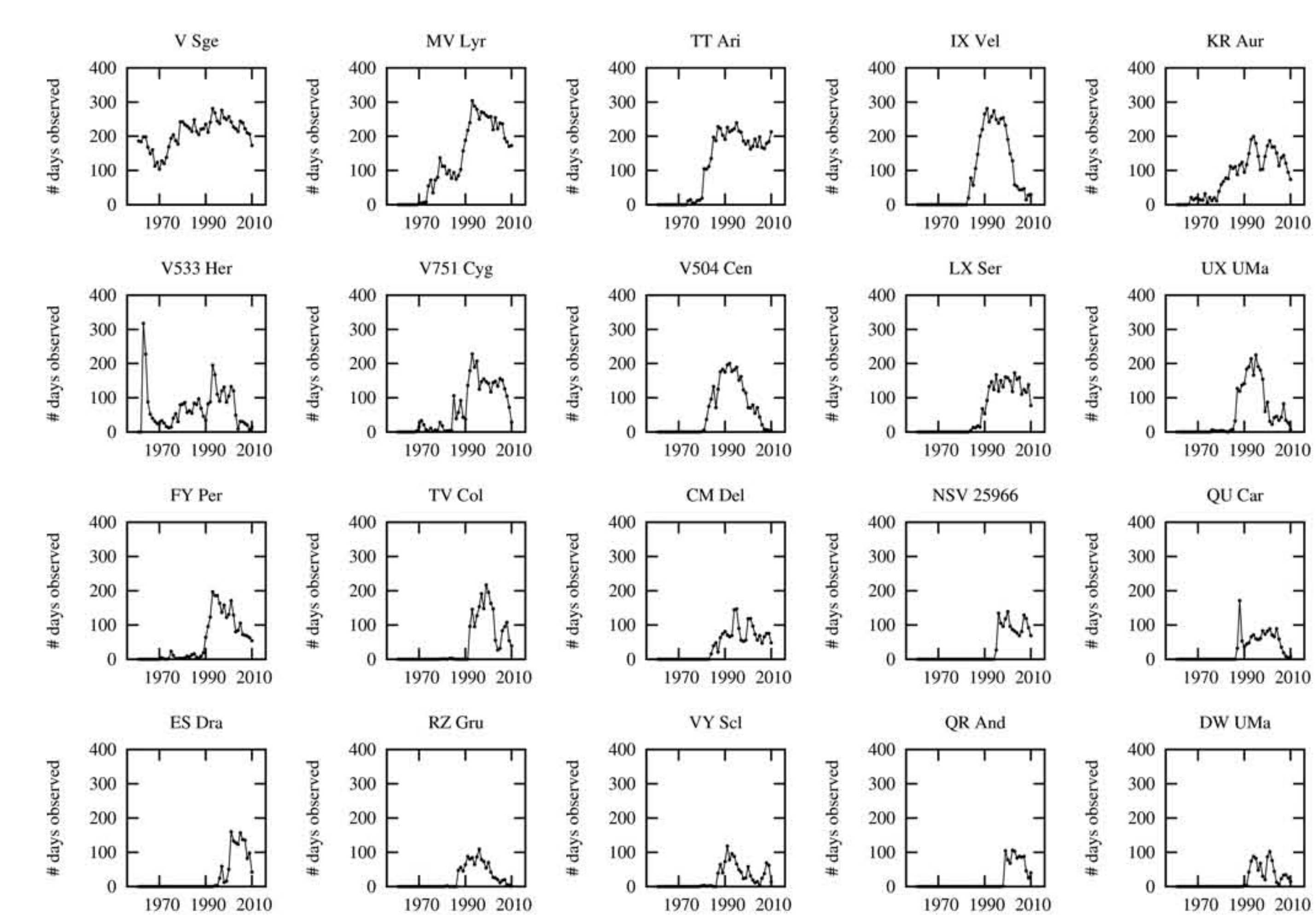
Figure 7: The 20 best-observed novalike cataclysmic variables. Only V Sge has good coverage throughout the 50-year span of this study, and the vast majority of these objects were discovered within the past 50 years. Observations of these sources peaked in the 1990s due to the interest generated from space-based X-ray observations in the 1970s-1990s.
