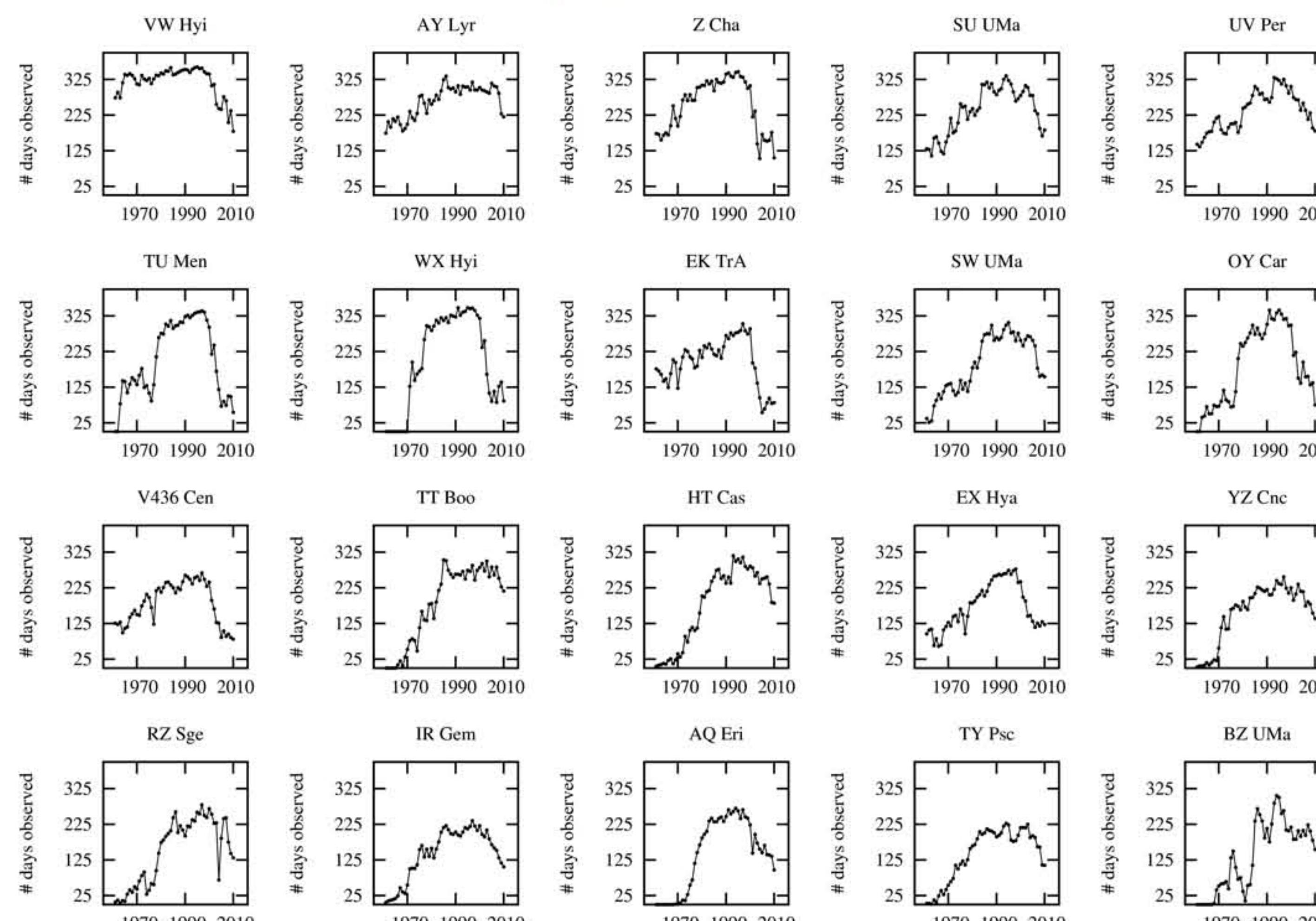
Figure 4: The 20 best-observed dwarf novae of type UGSU (SU UMa-type). Many of these stars show significant declines in coverage starting in 2000.
