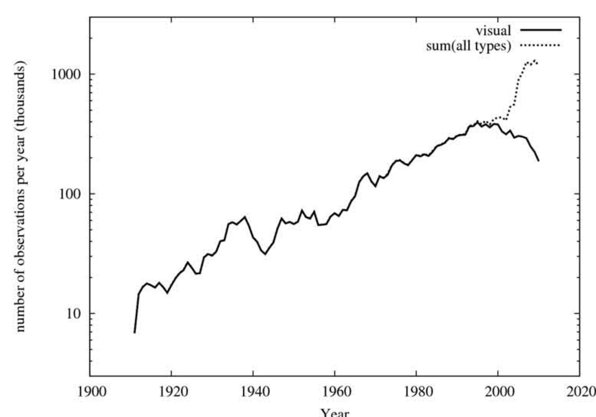
Figure 1: The number of observations per year found in the AAVSO International Database (AID): solid line , visual data; dotted line , all data. These numbers include data from the AFOEV and RASNZ. Beginning around the year 2000, CCD observations became the majority of observations submitted per year. The number of visual observations has been in decline since its historical maximum in 1995.
