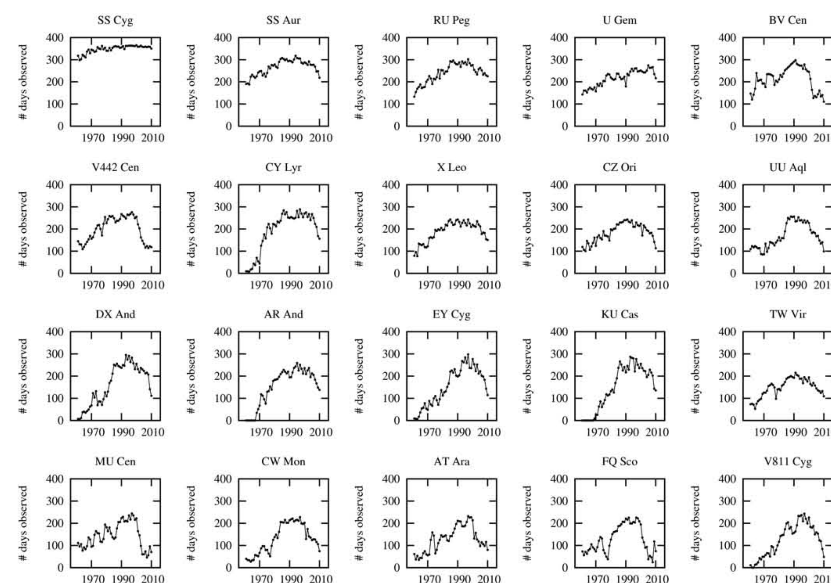
Figure 3: The 20 best-observed dwarf novae of type UGSS (SS Cyg-type). Several of these stars have been observed for many decades, with the longest-observed star being SS Cygni itself (SS Cyg is one of the best-observed stars in the AID, with nearly 365 days of coverage per year). The remainder of the 20 show declines in coverage of varying degree.
