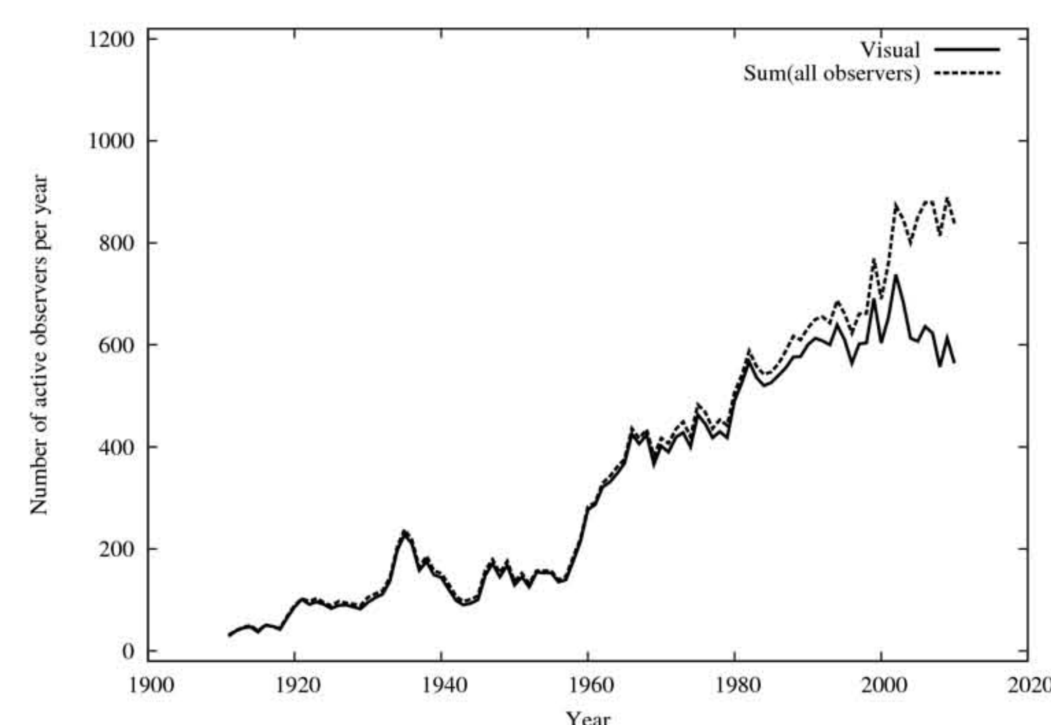
Figure 2: The number of observers whose data are submitted to the AID per year: solid line , visual data; dotted line , all data. Visual observers -- including those who also observe with a CCD part of the time -- still represent a majority of observers. Recent trends suggest the number of observers is holding steady or declining slightly.
