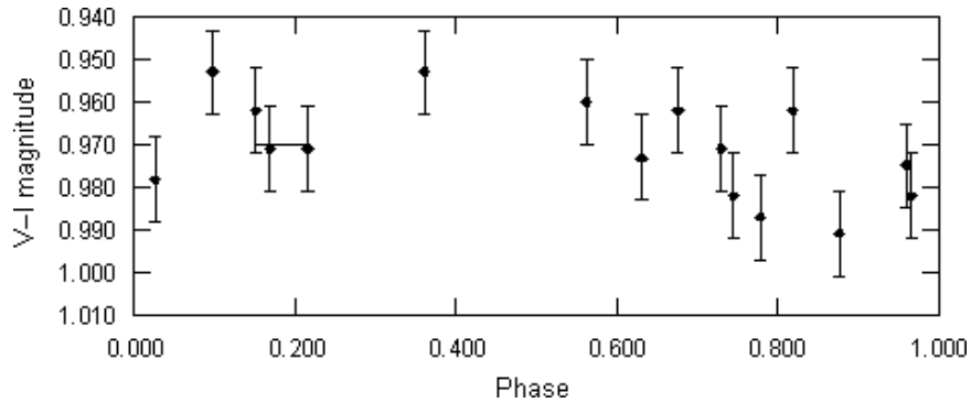
Figure 8. V-I data for V478 Lyr, for the third data segment. From observations by the author in 2005. Error bars are \pm 0.01 magnitude.
