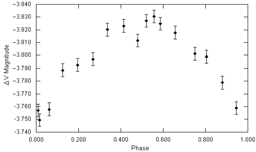
Figure 1. Photometric variation of V478 Lyr for the first data segment, 29 June 2005–11 July 2005. From observations by the author in 2005. Error bars are \pm 0.005 magnitude.
