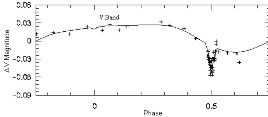
Figure 6. Data fit for a two-spot model for V478 Lyr, for the second data segment. From observations by the author in 2005. Spot 1: Longitude, 24; Latitude, 32; Radius, 16; Dimming, 0.901. Spot 2: Longitude, 100; Latitude, 48; Radius, 10; Dimming, 0.891. \chi -square = 1.07.
