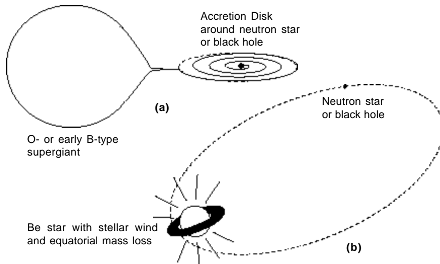
Figure 1. Schematics showing the two main types of high mass X-ray binaries. (a) A short period (days) SG/X-ray binary consisting of a supergiant O- or early-B type star filling or nearly filling its Roche lobe and transferring mass via an accretion disk to an orbiting neutron star or black hole. (b) A long period (several weeks to several years) Be/X-ray binary consisting of a Be rapidly rotating main sequence star that transfers mass to a neutron star or black hole in a highly eccentric orbit via mass loss through stellar wind and through a centrifugally produced equatorial disk.
