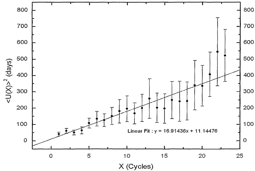
Figure 1. Graph of \langle u(x) \rangle^2 vs. x of \alpha Ceti (weight = sample size). The \langle u(x) \rangle diagram for about thirty cycles of Mira. Note that the error bars become larger as x becomes larger, because there are fewer and fewer pairs of (O-C)s that are x cycles apart.
