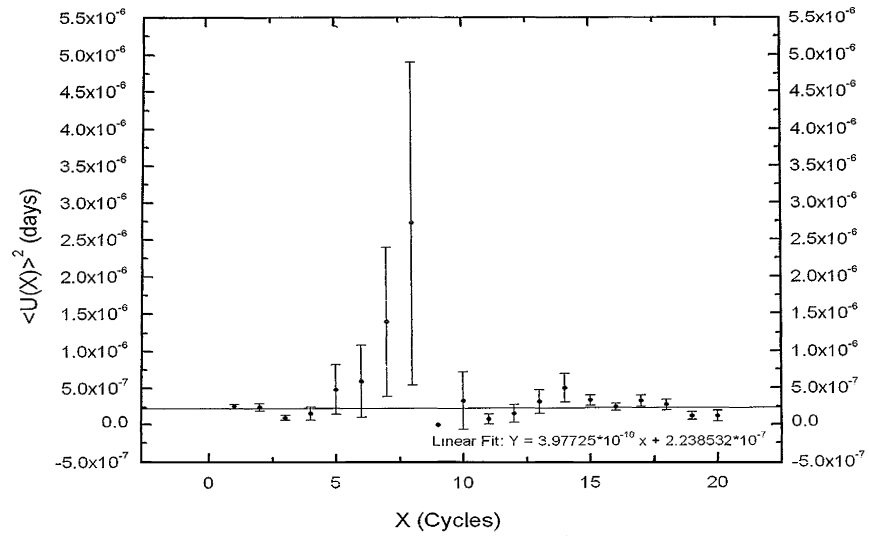
Figure 2. The \langle u(x) \rangle diagram for CY Aqr. The best-fit line is almost horizontal, indicating that the cycle-to-cycle period fluctuations (represented by \varepsilon ) are negligible.
