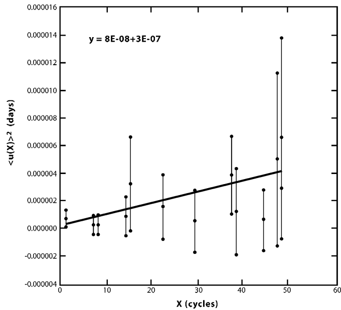
Figure 3. The \langle u(x) \rangle diagram for XX Cyg. The best-fit line has a positive slope that is significant at the 3\text{-}\sigma (standard deviation) level, indicating that the cycle-to-cycle period fluctuations (represented by \varepsilon ) are present and significant.
