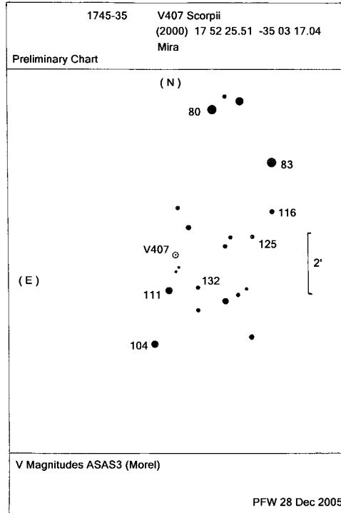
Figure 1. Identification chart for V407 Sco, adapted from RASNZ charts (Bateson et al. 1960; Bateson and Morel 1986).
