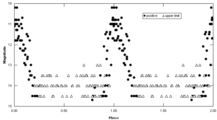
Figure 2. V407 Sco phase plot based on a 401.5-day period and using the author's data.
