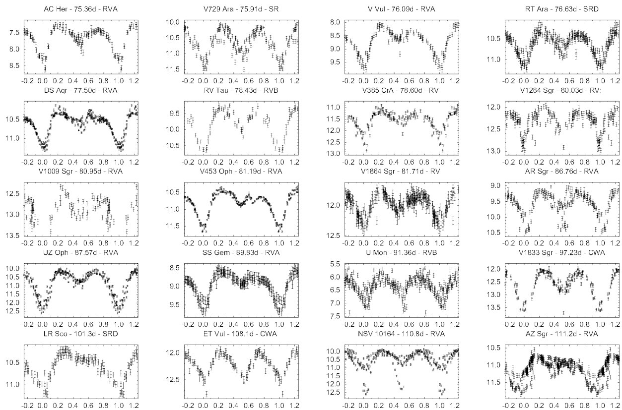
Figure 1, continued. Phase plots for CWA and RVA variables from ASAS-3 data. (Continued on following page.)
