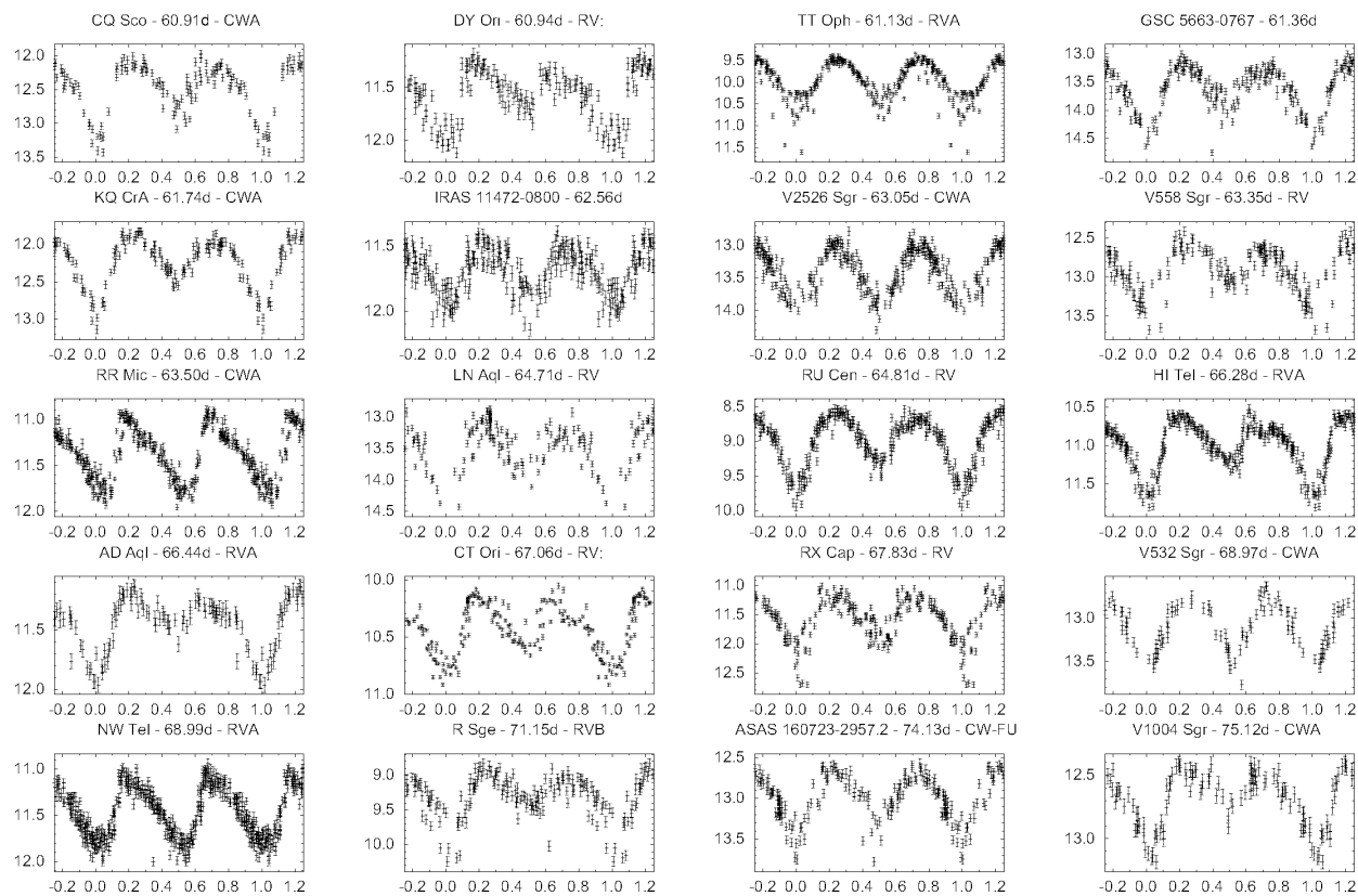
Figure 1, continued. Phase plots for CWA and RVA variables from ASAS-3 data. (Continued on following pages.)
