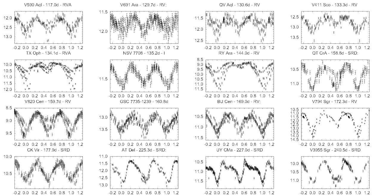
Figure 1, continued. Phase plots for CWA and RVA variables from ASAS-3 data.
