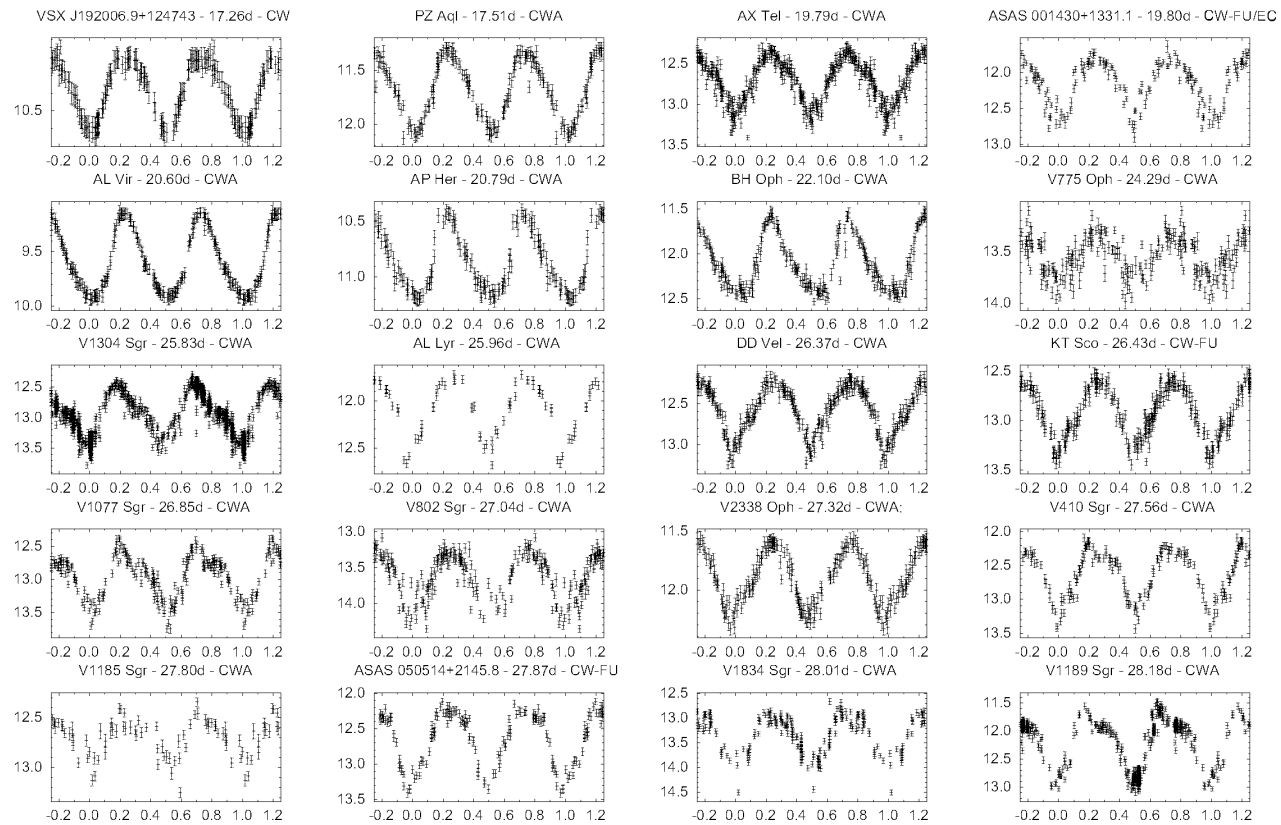
Figure 1. Phase plots for CWA and RVA variables from ASAS-3 data, arranged by period. (Figure continued on following pages.)
