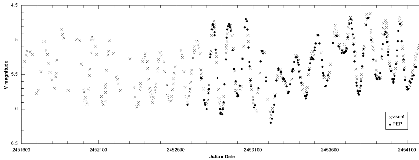
Figure 3. New visual and photoelectric photometry observations of \theta Aps with a correction of -0.05 magnitude applied to the visual estimates.
