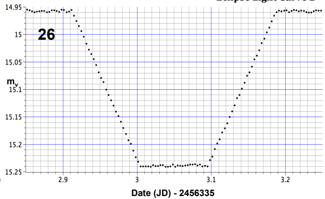
Eclipse Light Curve 2
