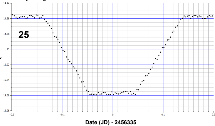
Eclipse Light Curve 1
