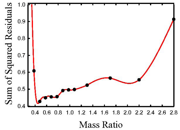
Figure 5. Mass ratio ( q ) search, fixed q -solutions vs. sum of square residuals to determine the best q -value.
