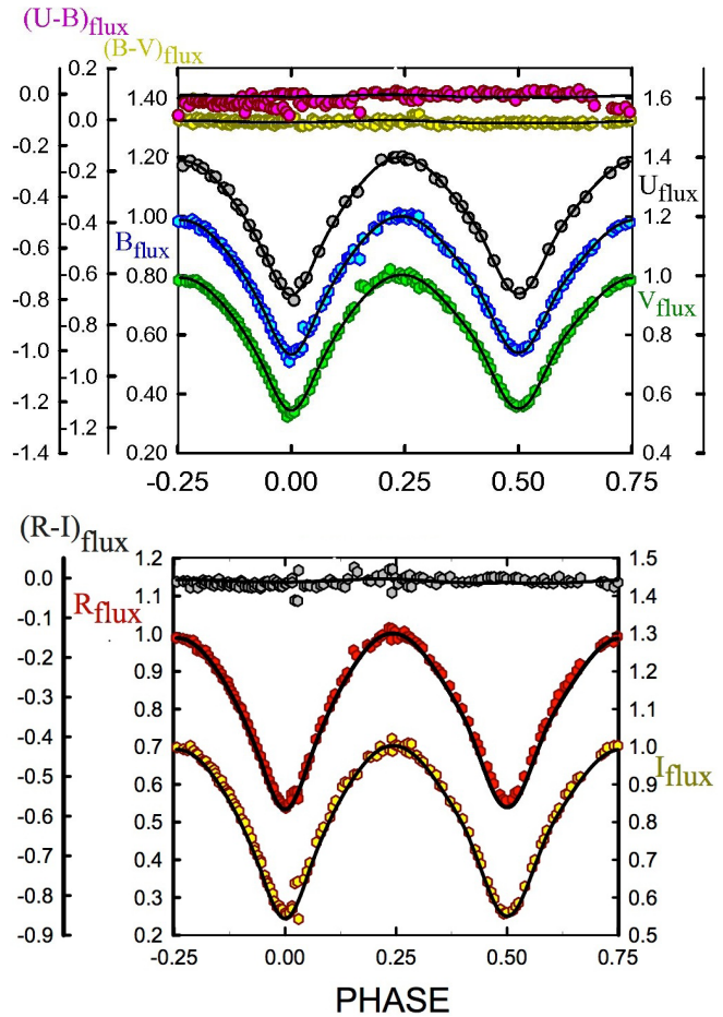
Figure 6a (top). U, B, V normalized flux curves overlain by our solution. Figure 6b (bottom). R, I normalized flux curves overlain by our solution.
