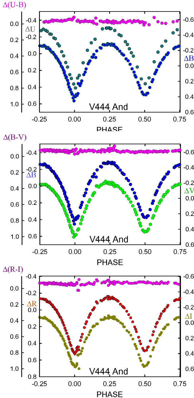
Figures 4a (top), 4b (middle), 4c (bottom). Phased \Delta U , \Delta B , \Delta V , \Delta R , and \Delta I differential magnitude light curves and \Delta(U-B) , \Delta(B-V) , \Delta(R-I) color curves.
