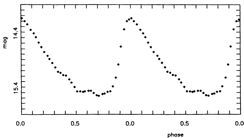
Figure 4. Phase averaged light curve from the observations in Figure 3.
