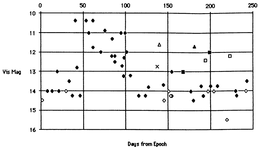
Figure 1. The light curve of TX Sgr from visual estimates reported in this paper, phased according to the ephemeris, T = \text{JD}2446792 + 246.7 \text{ E} . Solid diamonds are estimates that seem to follow the expected light curve, while other symbols indicate minima that were brighter than expected.
