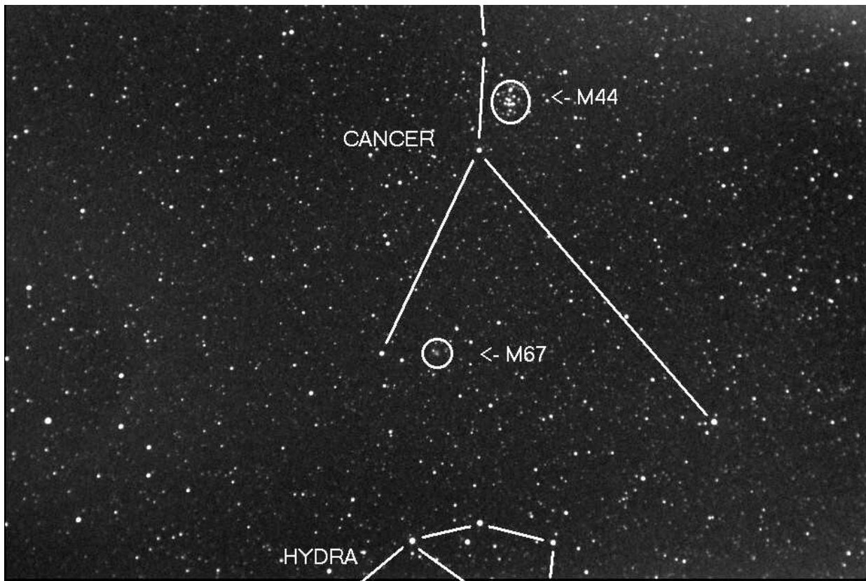
Figure 13. Southern part of the constellation Cancer and northern part of constellation Hydra. M67 is a "smudge" at this resolution (160 "arc). The image covers an area 27.2 \times 18.1 degrees.
