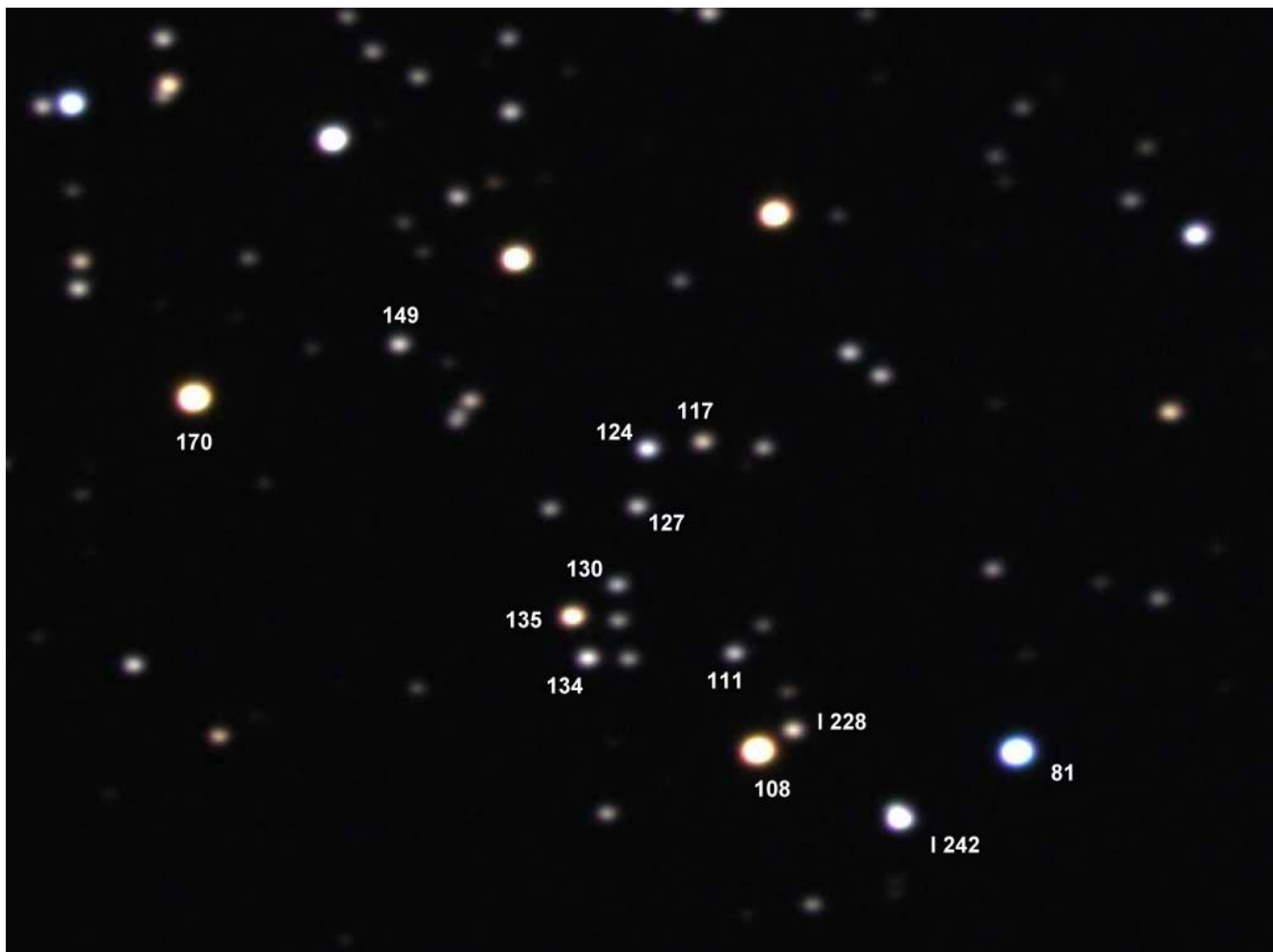
Figure 18. Zoom of central region of the previous image. Star #135 has coordinates 8:51:22,+11° 46' 06" (epoch 2000.0). The image area is 6.82 x 4.85 'arc. The FWHM resolution is 4.0 "arc in this sum of several 1-minute unguided exposures using BVR filters. The faintest stars have a visual magnitude of about 14. Stars to be used by AAVSO observers are indicated with star numbers. The bluest star is #81 and the reddest is #108. [LX200 10-inch SCT, f/6.3, SBIG ST-8E, True Tech filter wheel w/ Schuler BVRI filters; 2002.04.22Z, Santa Barbara,CA.]
