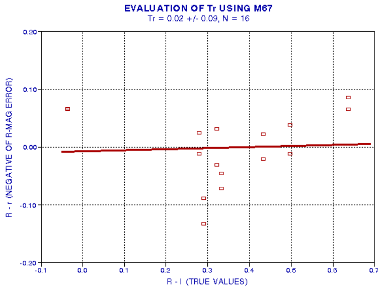
Figure 9. The same measurements are used to show that a correction is required to convert measured "r" to true "R" and that this correction depends on the star's R-I color. The LS fitted slope of the data graphed here corresponds to coefficient T_r .
