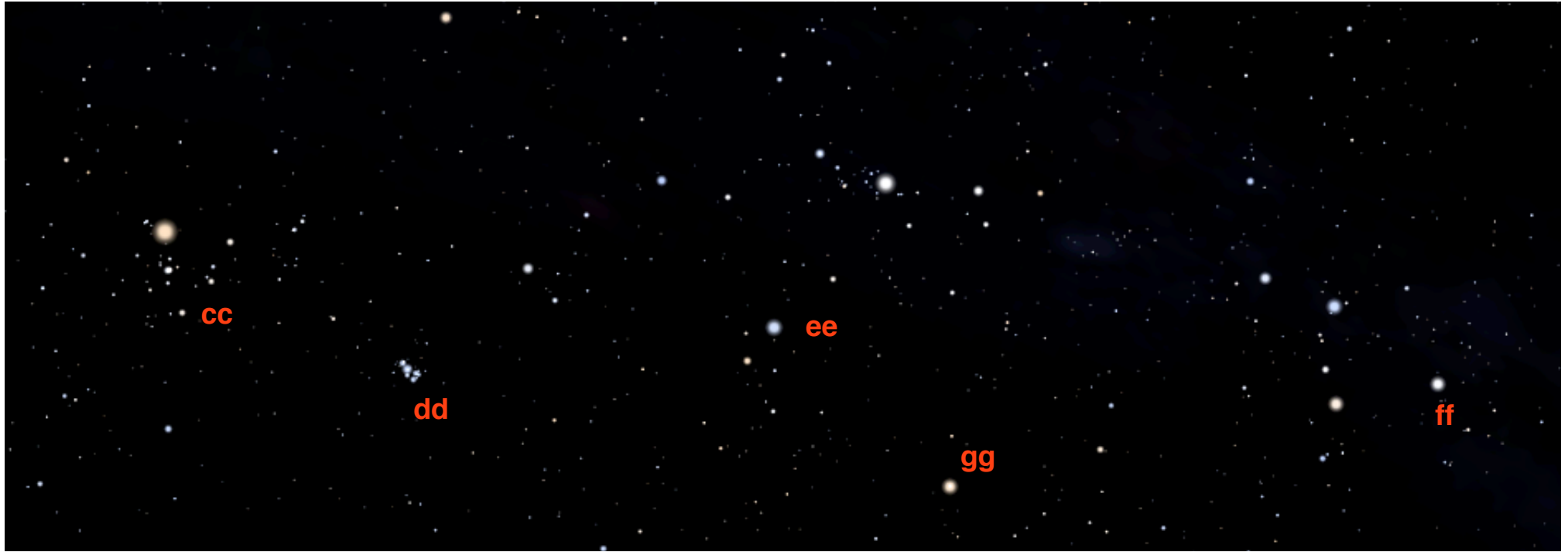
Star Map 7:
