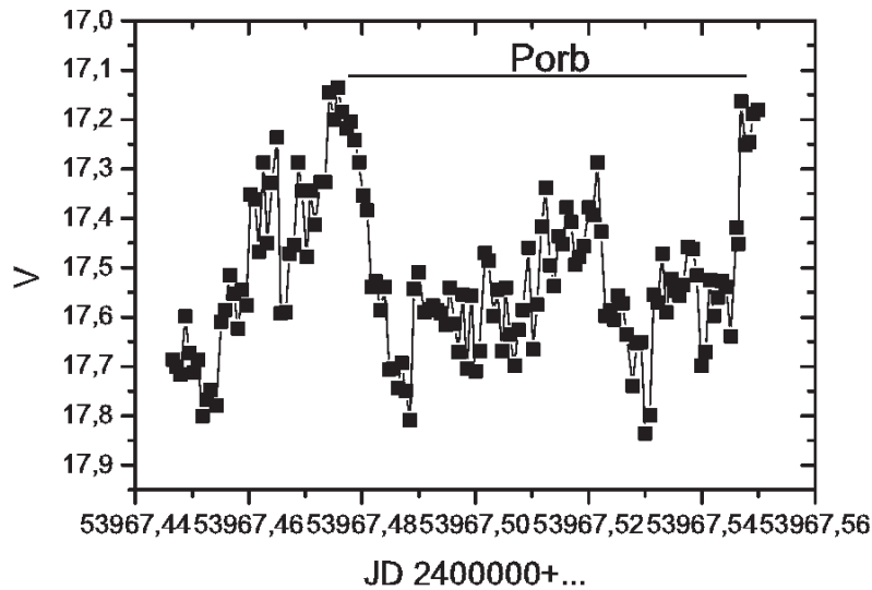
Figure 2. Light curve of V1504 Cyg showing a two-humped structure in minimum. The 2.6-m Shajn telescope of CrAO in 2006 revealed the unequal humps of 0.6 and 0.4 magnitude in V . The lesser-amplitude and short-term QPOs are superimposed on the orbital light curve.
