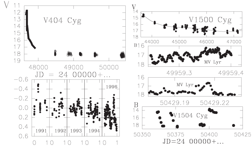
Figure 1. The light curves of V404 Cyg outburst and decline, V1500 Cyg decline, V1504 Cyg outbursts and superoutburst, and the behavior of MV Lyr during two selected nights in the low brightness stage. The brightness decline for V404 Cyg (solid line) is taken from numerical observations; our data are marked by circles. In the bottom panel, data folded on the orbital period are shown.
